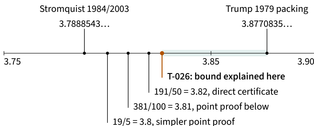
Figure 3. Bounds on s(11) . The shaded band is the gap left by the certificates explained here. At T-026's bound the gap is 0.0506361\dots wide, down from 0.0882292\dots at Stromquist's bound. T-060, by Queuingtheorydotcom after Levy et al. 2026, closes the remaining gap: its independently checked lower bound equals Trump's upper bound at the exact algebraic side T . 3.8770835\dots is a truncated decimal display of T .
